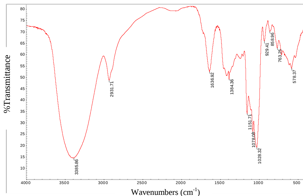
Figure 13. FT-IR spectrum of the black garlic nanoparticles system was synthesized at rate \frac{1}{2}
